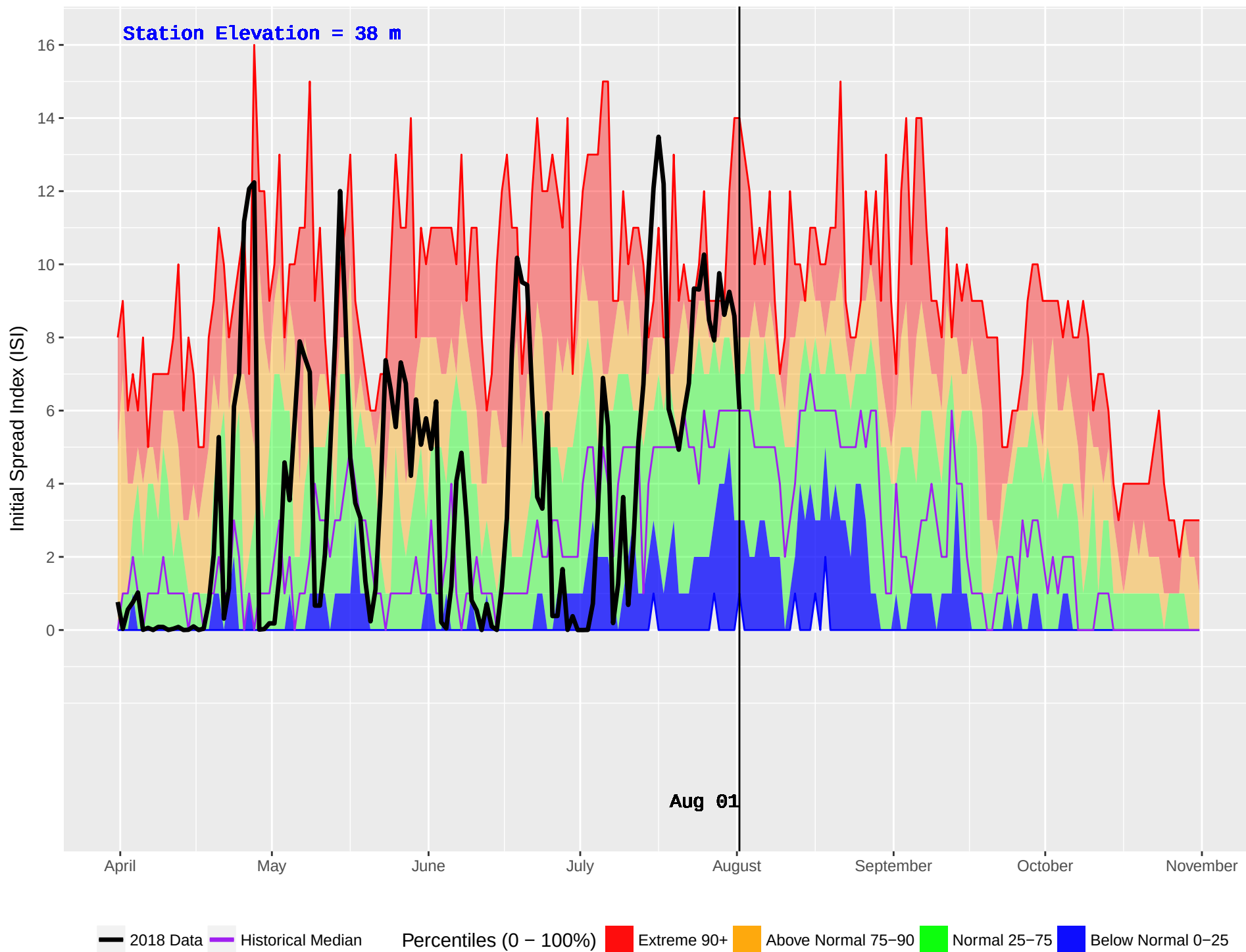
HAIG CAMP (67) : Historical (2002–2016) and Current (2018) Daily Initial Spread Index (ISI)
