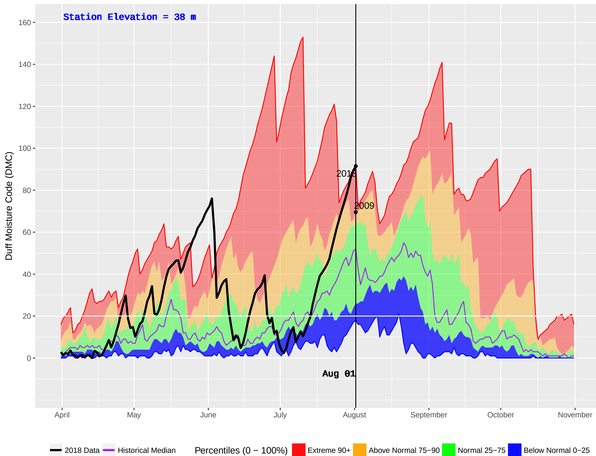
HAIG CAMP (67) : Historical (2002–2016) and Current (2018) Daily Duff Moisture Code (DMC)
