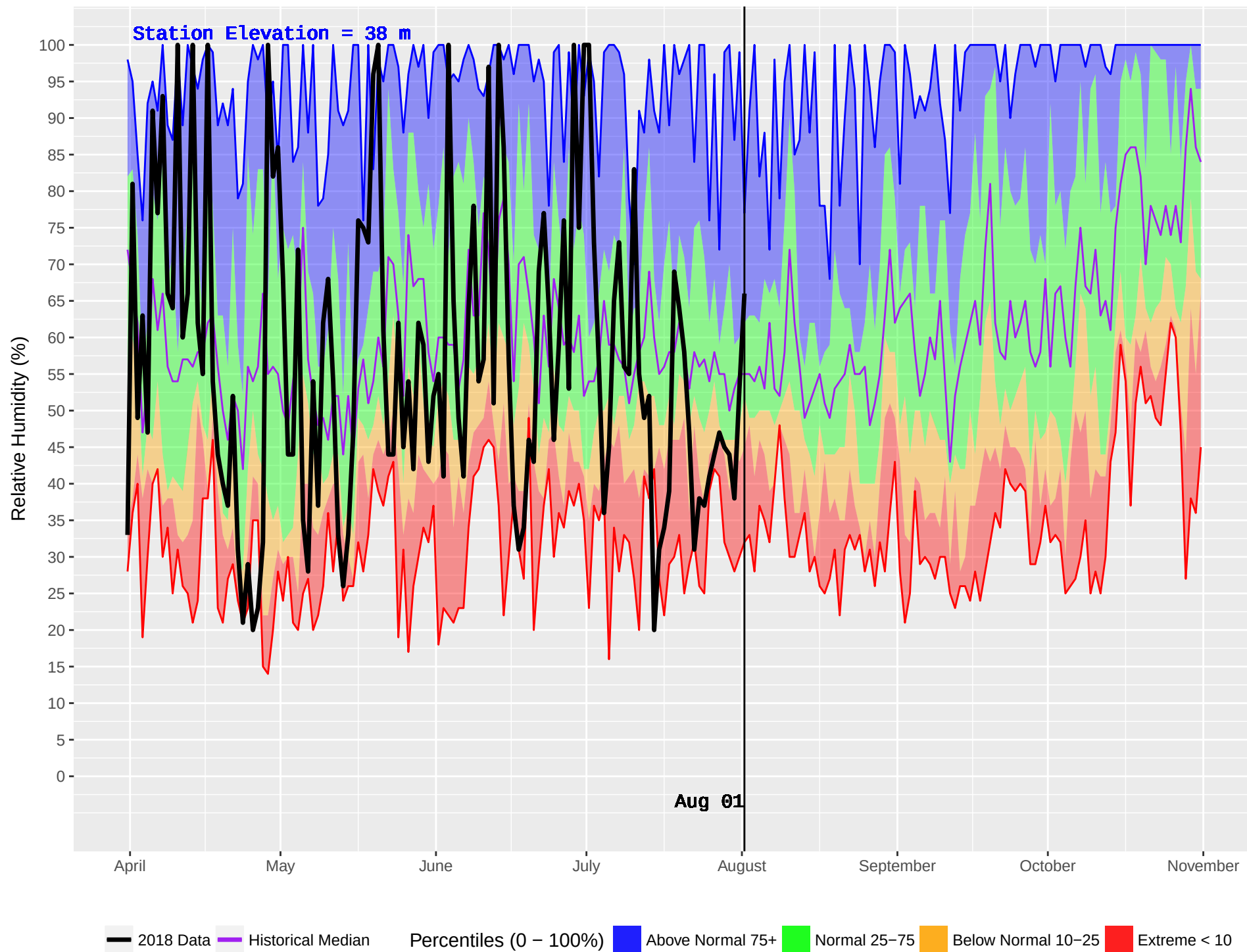
HAIG CAMP (67) : Historical (2002–2016) and Current (2018) Daily Relative Humidity
