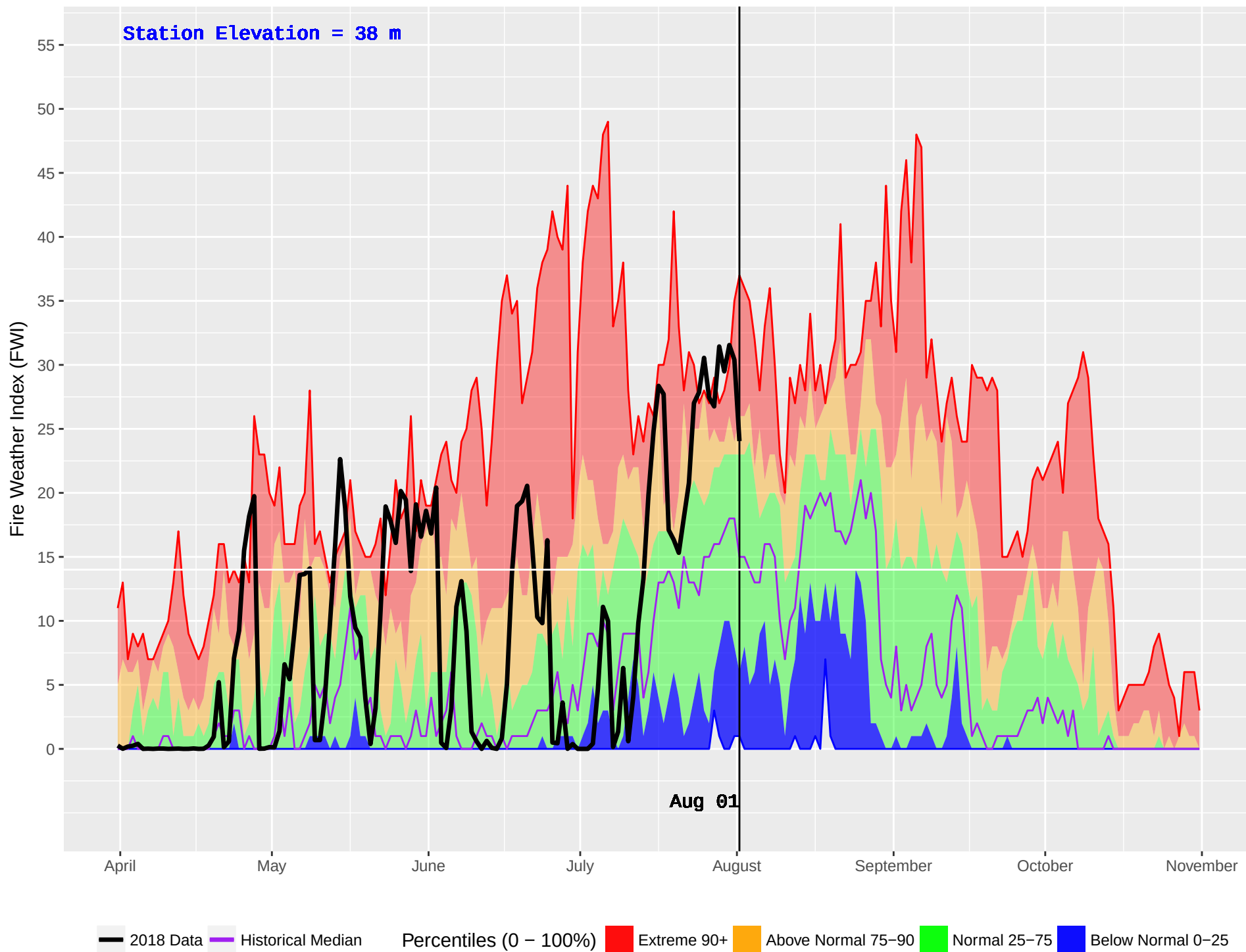
HAIG CAMP (67) : Historical (2002–2016) and Current (2018) Daily Fire Weather Index (FWI)
